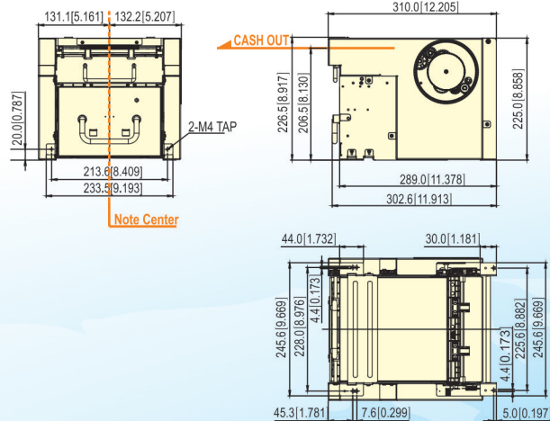
NDR1000
